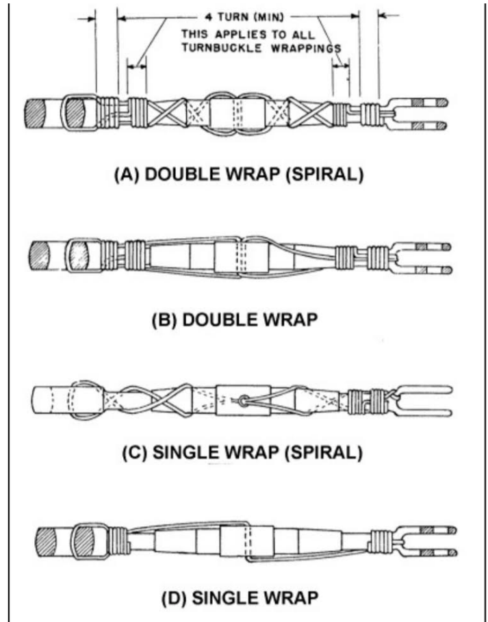
FIGURE 7-26. Safelying turnbuckles.
