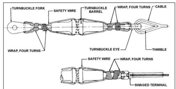
FIGURE 7-27. Securing turnbuckles.
